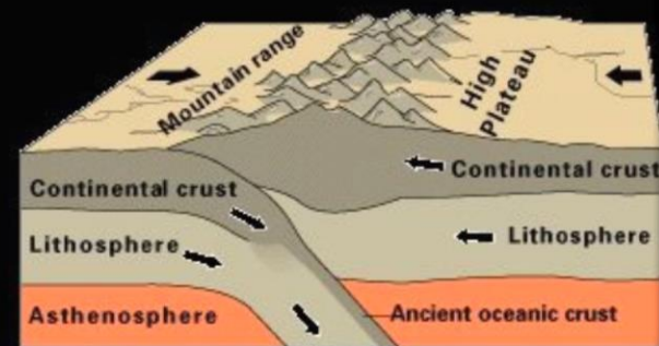
Continental-continental convergence
