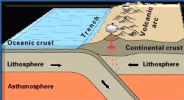
Oceanic-continental convergence
