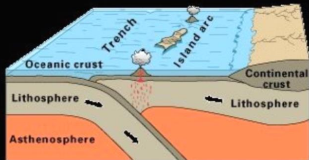
Oceanic-oceanic convergence
